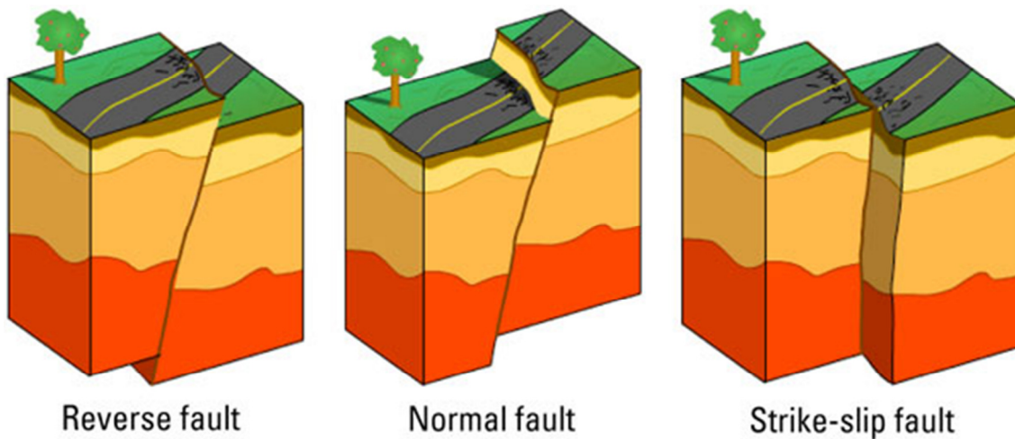
Fault types (from IUGS)
