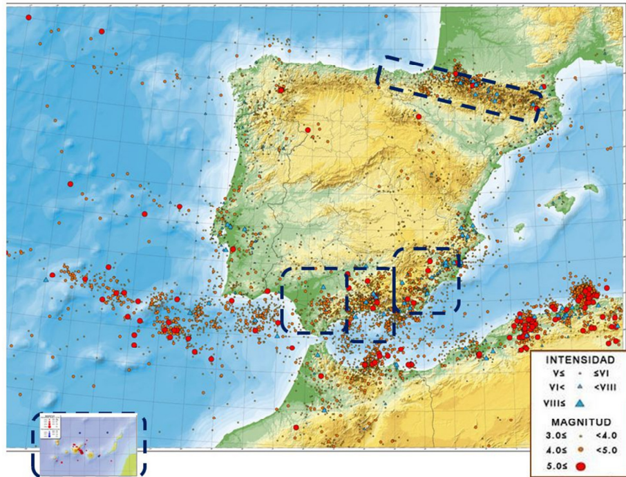
Seismicity map for Spain (IGN) link
