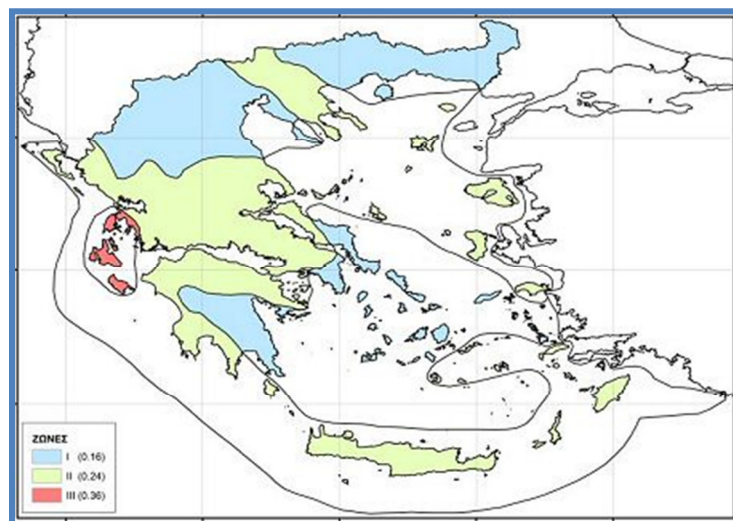
Figure 1: Greek Seismic Hazard Map
