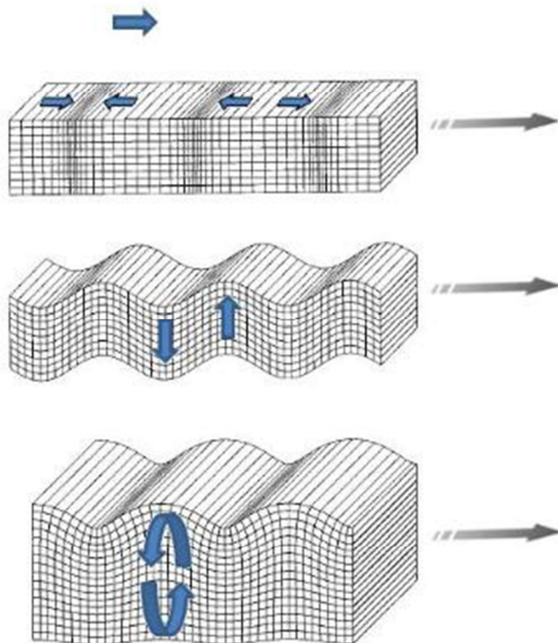
Seismic waves: Upper image P waves, middle image S waves and lower image surface waves
