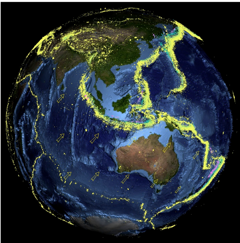
Earthquake epicenters in the Pacific area
