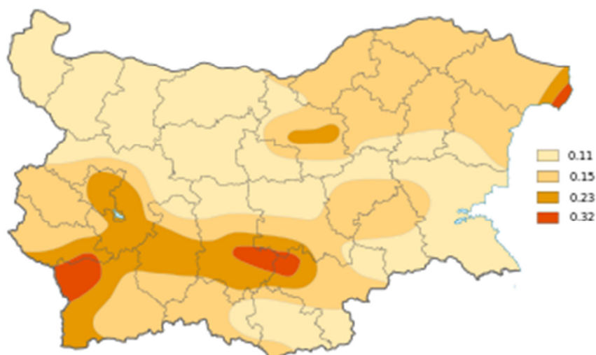
(Fig.1) Seismic risk map, showing maximum values of acceleration of the Earth surface (measured in g) with a repetition time of 475 years.
