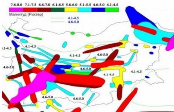
Fig. 6 Map of possible seismic focus in Bulgaria (PSF)
