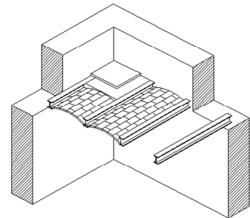
Iron "I" beams and brick arches floor
