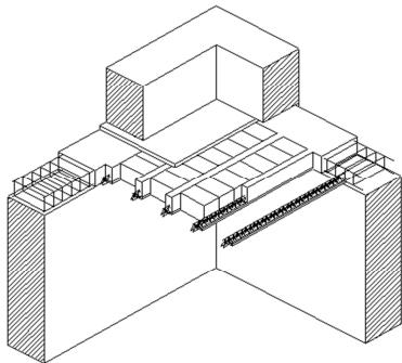
Floor with reinforced concrete ring beam
