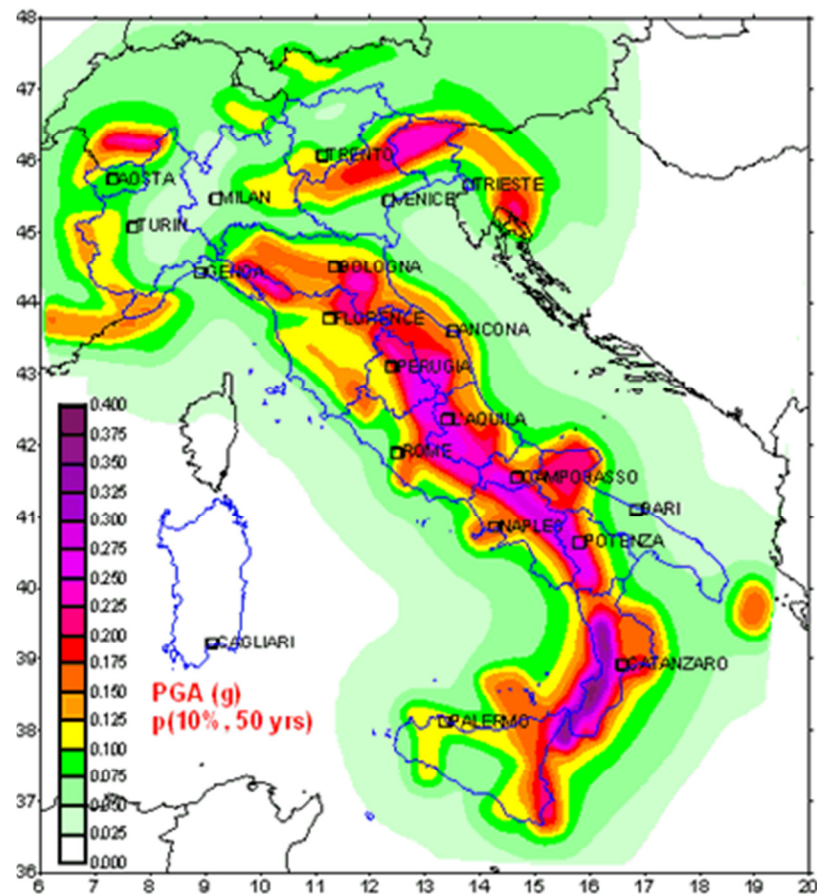
Figure 2: Italian Seismic Hazard Map
