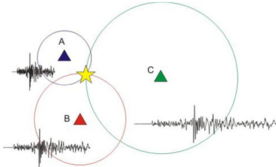
Locating an earthquake epicentre (star) by three seismograph stations (A,B,C) by the British Geological Survey ( http://www.bgs.ac.uk/discoveringGeology/hazards/earthquakes/locatingQuakes.html )
