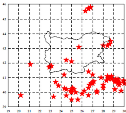
Fig. 5 Documented earthquakes with magnitude 7.0 and higher
